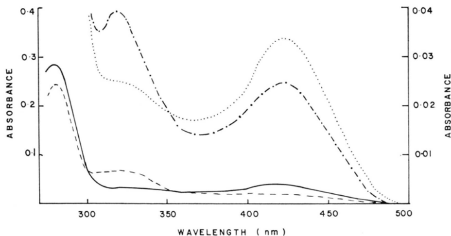
Fig. 1. Absorption spectra of pure 5-aminolevulinatase synthase in the presence of PLP and after treatment with \text{NaBH}_4 or 2-mercaptoethanol. Apoenzyme (0.4 mg/ml) in 0.05 M potassium phosphate buffer, pH 7.2, having equivalent or excess of PLP (solid line). The buffer blank contained equal amount of PLP. The enzyme-PLP complex after reduction with 0.005 M \text{NaBH}_4 at neutral pH and dialysis against 0.05 M potassium phosphate buffer, pH 7.2 (broken line). The dotted line represents the enzyme-PLP complex on a 10-fold expanded scale; the effect of adding 0.05 M 2-mercaptoethanol to the enzyme-PLP complex is represented by the dashed-dotted line which is also on a 10-fold expanded scale.
